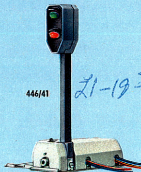
446/41 Colour-light Home Signal · Light change from red to green; lighting by No. 485 bulbs, red and green · Extra lever for manual operation of signal · Width 1½ in., length 2¾ in., height 3¼ in.
