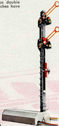
7041 $ 7.50 Home signal with two semaphore arms, not coupled together. Operation, connection and traction current regulation as for all signals with train control action, but with an extra third solenoid. The current returns through an additional blue cable with an orange cross-plug connector. The three signal indications possible through coupling the two armatures together mechanically are obtained by energising one coil only. Light changes from red to green or from red to green/amber. Width 1 1/8 in.; length 3 3/8 in.; height 5 in.
