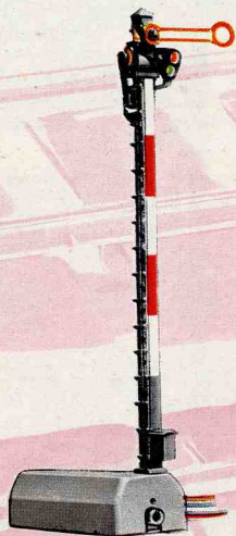
7039 $ 4.95 Home signal with one semaphore arm; light changes from red to green. Width 1 1/8 in.; length 2 3/4 in.; height 5 in.
