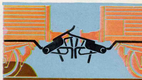
The new design of coupling allows the train to be shunted further after the uncoupling device has operated, without the couplings engaging again.
