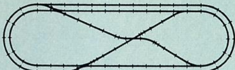
Double-track oval with double reversing loop
