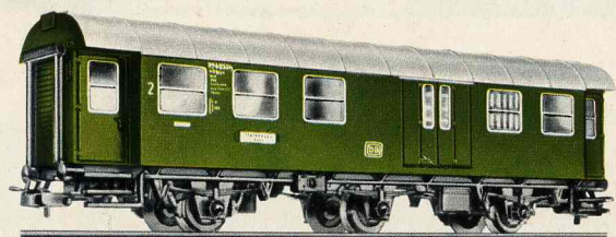
4080 PASSENGER CAR WITH BAGGAGE COMPARTMENT · Second class, six-wheeled coach · A model of the German Federal Railways type BD3yge · Dark green body with inset plastic window frames · Simulated rubber diaphragms on ends · Silver roof · Length 6" · Provision for fitting the 7074 lighting equipment (see page 54)
