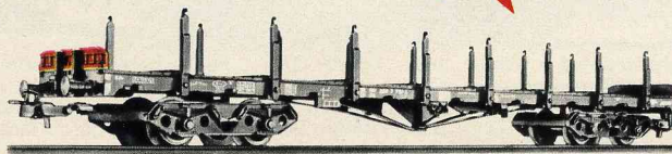
4663 FLAT CAR · Eight-wheeled · A model of the German Federal Railways Type SS1mas 53 · Die cast metal body, black with brown end sills · Side stanchions fold down · Length 9"
