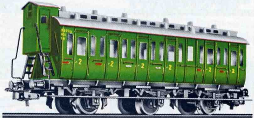
4005 COMPARTMENT COACH WITH BRAKEMAN'S CABIN · Six-wheeled with doors for six compartments · Designed to accept interior lighting 7074 · Clear plastic windows · Dark green body with grey roof · Length over buffers 5 1/4"
