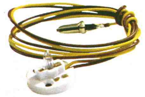
8950 Light socket with light insert and cable · For stations, buildings and the like
