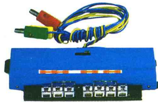
8945 Universal remote-controller with two single-pole switches and one change-over switch · Operating voltage 10 V · Double solenoid operation · Actuated by contact track sections, from a control panel or by means of an additional hand lever · Width 1 \frac{3}{16} " · Length 2 \frac{3}{4} " · Height \frac{3}{16} "
