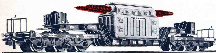
4617 Depressed center flat car · Loaded with a transformer · 10" long
