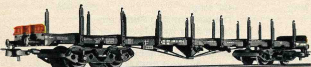
4663 Flat car · A model of the German Federal Railways' type SSImas 53 · Die-cast zinc body · Side stanchions fold down · 9" long
