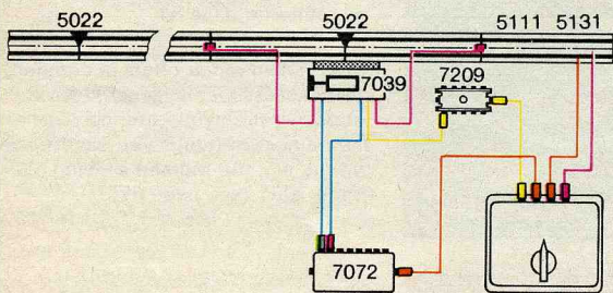
Connection of 7039 for track contact operation
