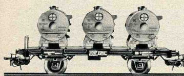
4520 Chemical container car · BAYER · Containers can be removed by crane 7051 · 4 1/4" long
