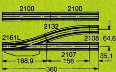
2108 Length = 35.1 mm (1 3/8")
