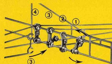
7006 Contact wire insu- lation · For insu- lating sections of contact wire from cross-spans · One required for each track and cross- span · 15x6 mm ( 5 / 8 "' x 1 / 4 "')
