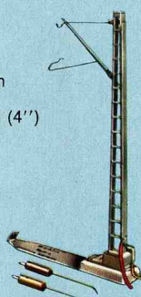
7201 Feeder mast for supplying current, with 2 permanently connected leads, one red, one brown · Additional brown lead · Built-in capacitor for radio interference suppression · One mast required for each electrical circuit · Instructions for setting up the catenary system are included · Height 100 mm (4")
