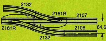
2106 Length = 168.9 mm (6 5/8")
