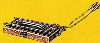
5112 Uncoupling track section for releasing automatic couplings · When the button on the control box is pressed, the solenoid-operated ramps on either side of the stud contacts are raised, releasing the couplings · 2 connecting leads · Length of track 90 mm (3 1/2")
